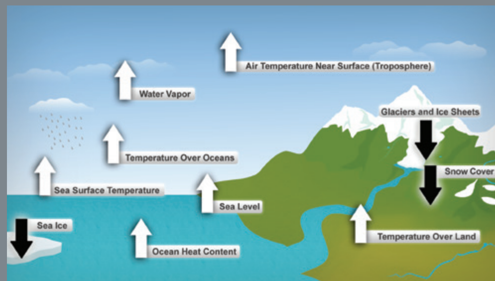
These are just some of the indicators measured globally over many decades that show that the Earth's climate is warming. White arrows indicate increasing trends; black arrows indicate decreasing trends. All the indicators expected to increase in a warming world are increasing, and all those expected to decrease in a warming world are decreasing. (Figure source: NOAA NCDC, based on data updated from Kennedy et al. 2010 a ).
