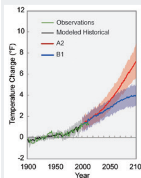
Different amounts of heat-trapping gases released into the atmosphere by human activities produce different projected increases in Earth's temperature. The lines on the graph represent a central estimate of global average temperature rise (relative to the 1901-1960 average) for the two main scenarios used in this report. A2 assumes continued increases in emissions throughout this century, and B1 assumes significant emissions reductions, though not due explicitly to climate change policies. Shading indicates the range (5 th to 95 th percentile) of results from a suite of climate models. In both cases, temperatures are expected to rise, although the difference between lower and higher emissions pathways is substantial. (Figure source: NOAA NCDC / CICS-NC).
